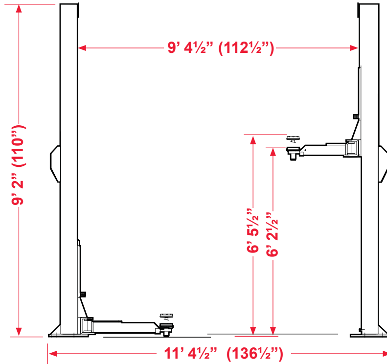
FIGURE 1 (Specifications Drawing)
