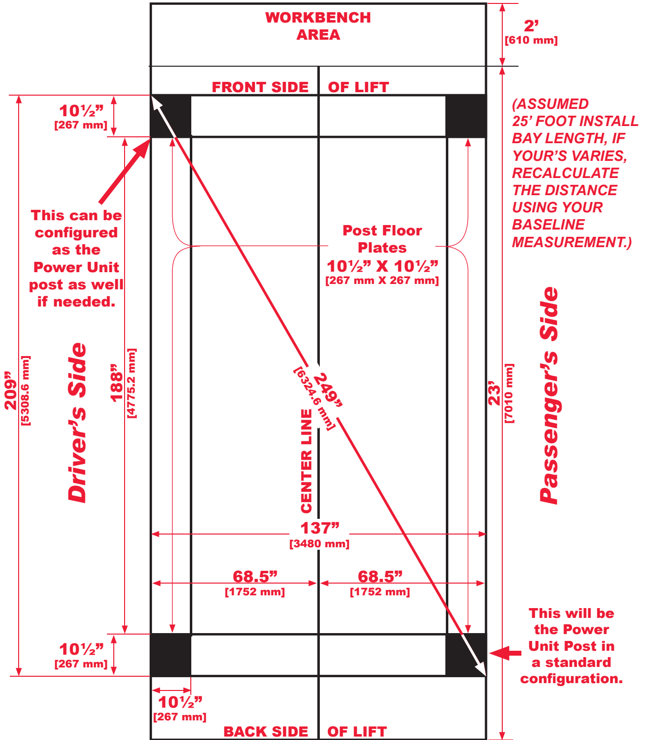
FIGURE 2 (Vehicle Lift Layout Drawing)
