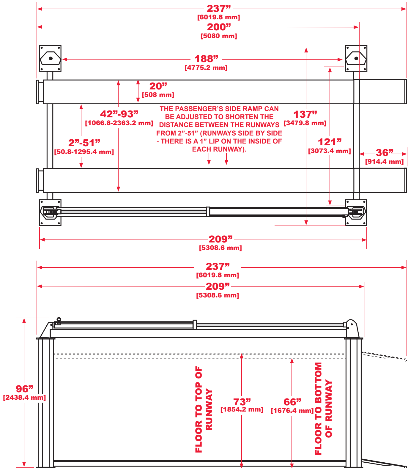
FIGURE 1 (Vehicle Lift Specification Drawings)
