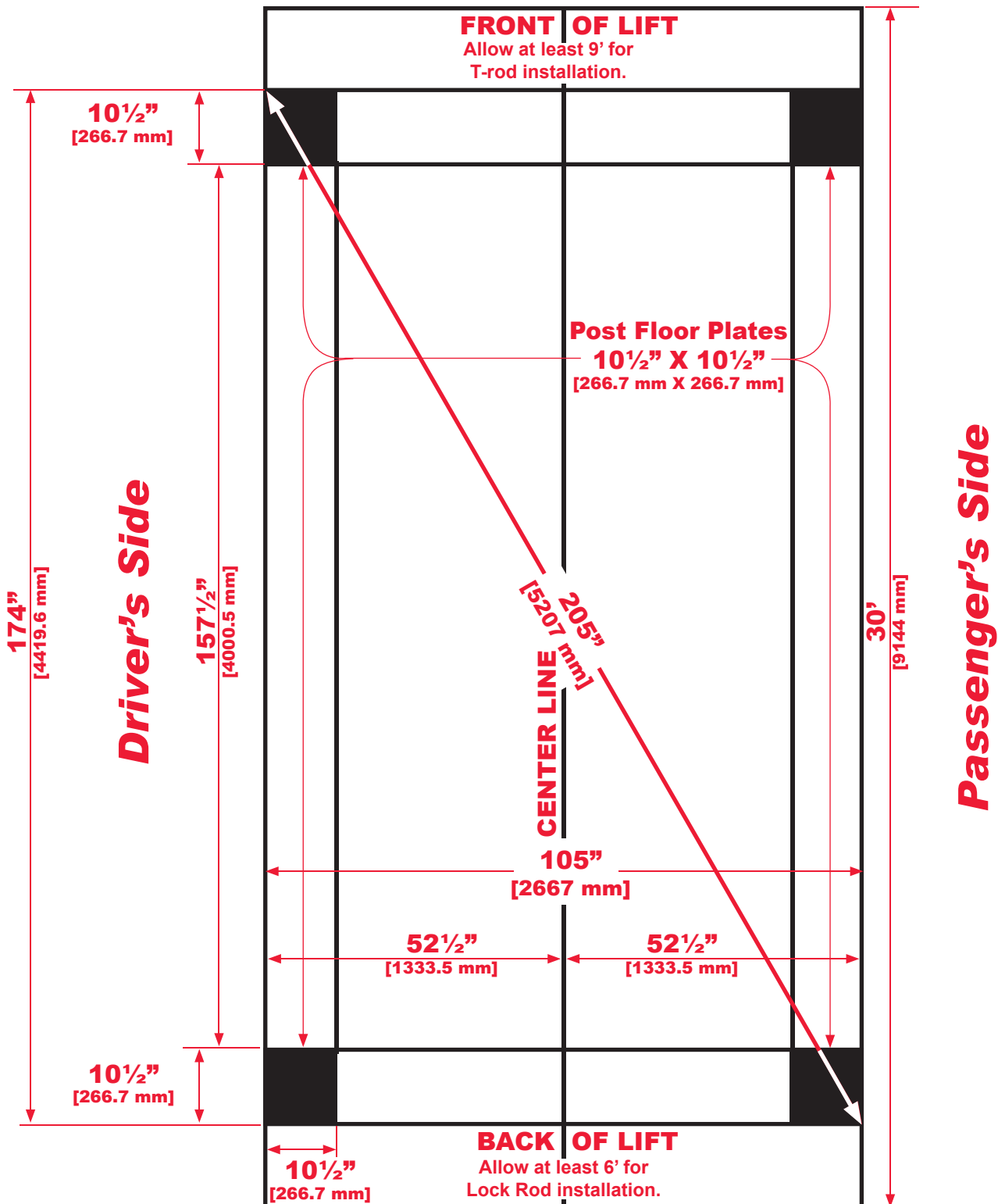
FIGURE 2 (Vehicle Lift Layout Drawing)
