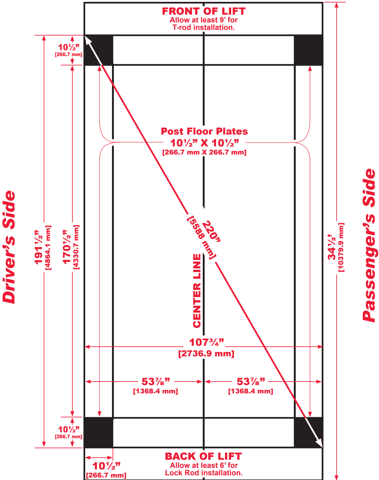
FIGURE 2 (Vehicle Lift Layout Drawing)
