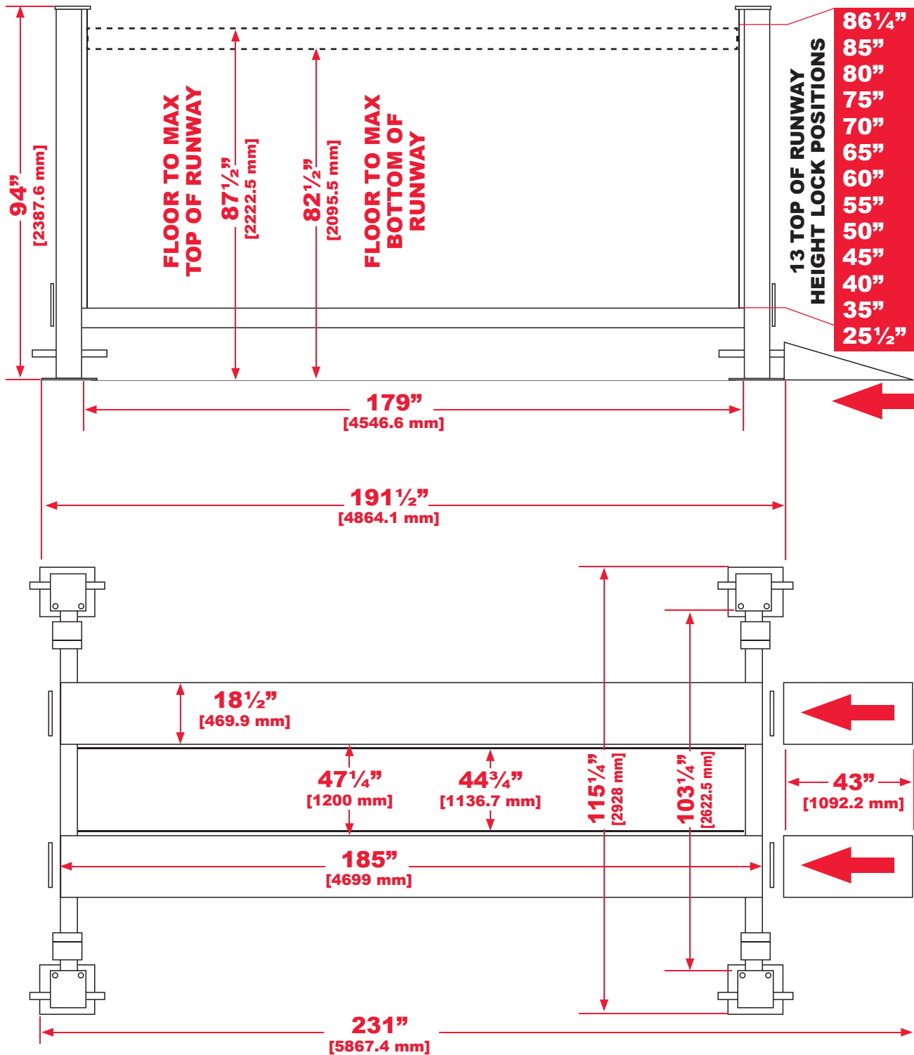
FIGURE 1 (Vehicle Lift Specifications Drawing)
