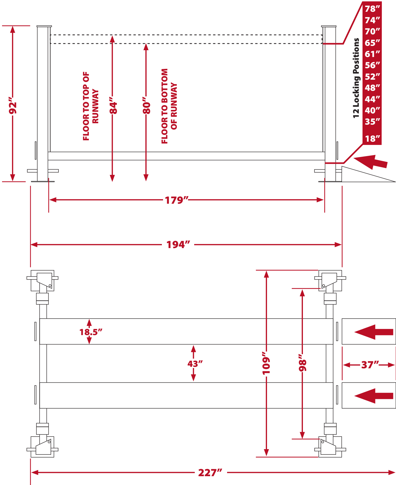
FIGURE 1b (CL 8,000 CSP XLT Specifications Drawing)
