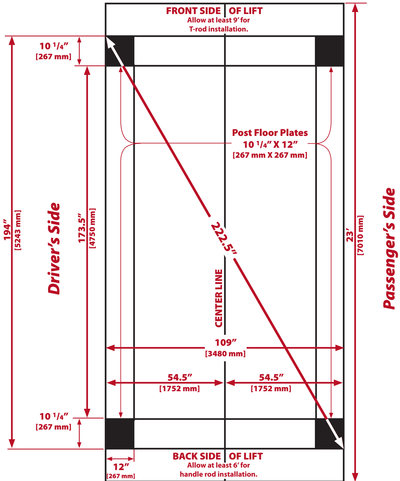
FIGURE 2b (CL 8,000 CSP XLT Layout Drawing)
